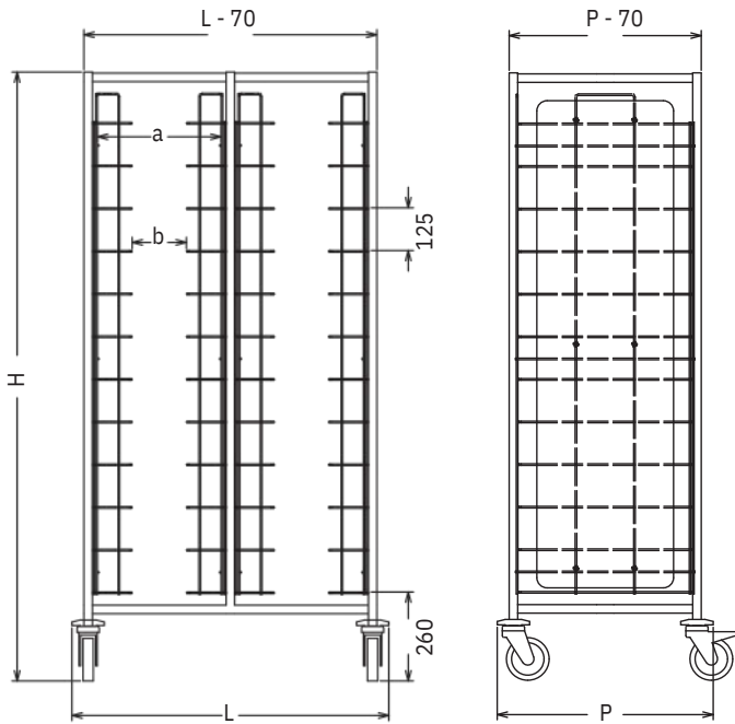
Trolley with 2x12 levels, insertion widthways (with two stacks, side by side). Front view.
